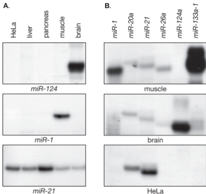
Fig. 2. Expression analysis of miRNAs in human tissues (A) and tissue-specific miRNAs (B) from 250 ng total RNA using the miRtect-IT™ miRNA Labeling and Detection Kit. The image was developed after 2 hr exposure.
