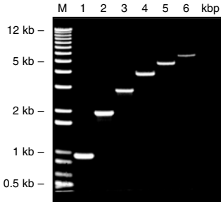
Fig. 1. DNA fragments ranging from 1 kb to 6 kb amplified from \lambda DNA.
